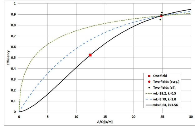
Fig. 4. Measured ESP efficiencies at KKAB with one and two fields in operation, together with curves from the Matts-Öhnfeldt equation for different values of the parameter k .
