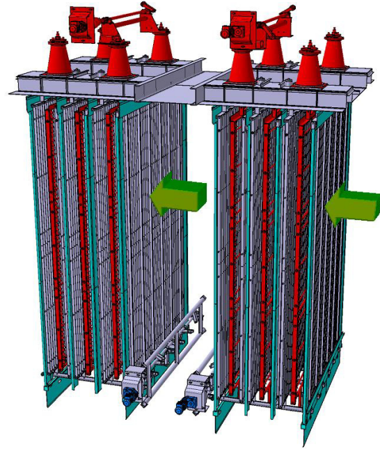
Fig. 3. Drawing of the internals of the cross flow ERDEC design ESP at KKAB power plant. The direction of the gas flow through the two fields is indicated by the green arrows.
