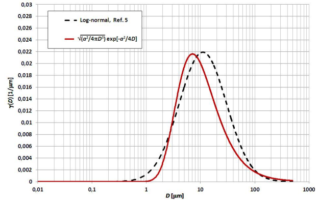
Fig. 2. Particle size distribution that results in the Matts-Öhnfeldt formula (with a^2 = 43 \mu\text{m}^2 ), compared to the log-normal distribution with same parameters as in Ref. [5].
